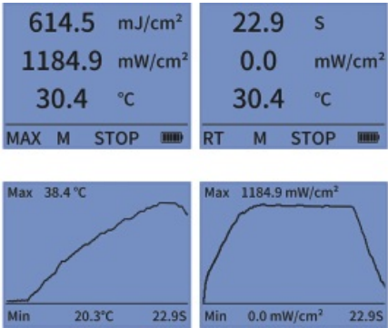
Simultaneous measurement of energy, power, and temperature with display of power curve and temperature curve (BGD 142)
