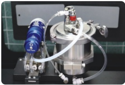
Spray gun
