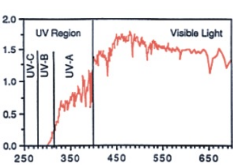
Distribution of Sun Spectrum
