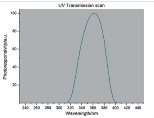
BGD142 Spectral Response Curve
