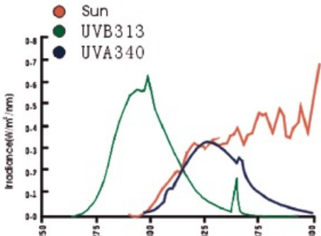
The Spectrum comparison of UV and Sun
